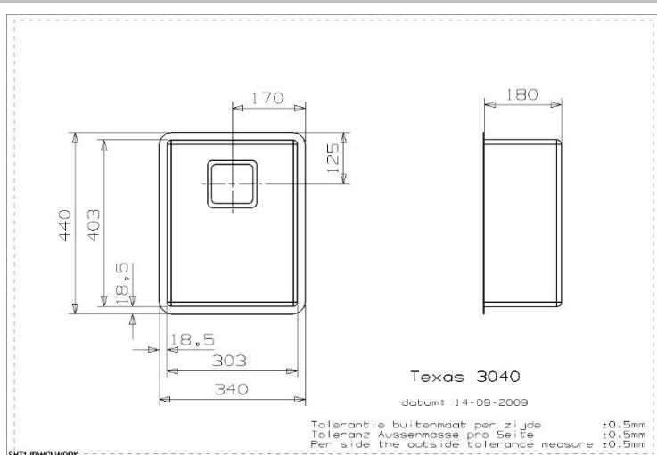
Inset cut-out
