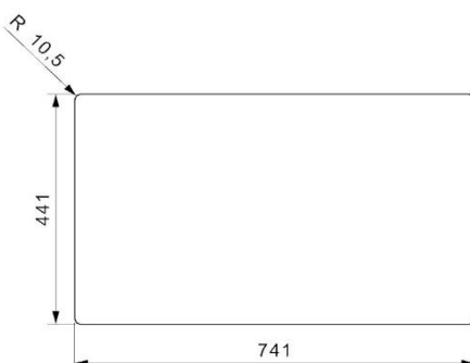
Flush cut-out
