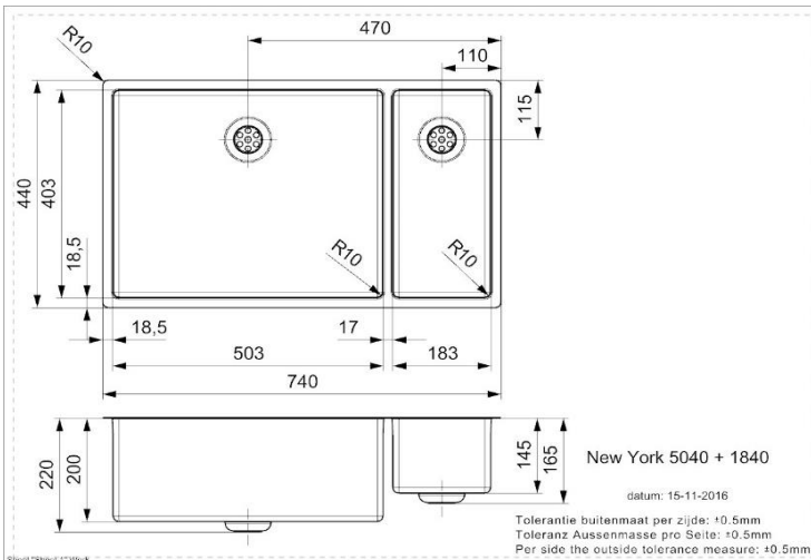
Inset cut-out
