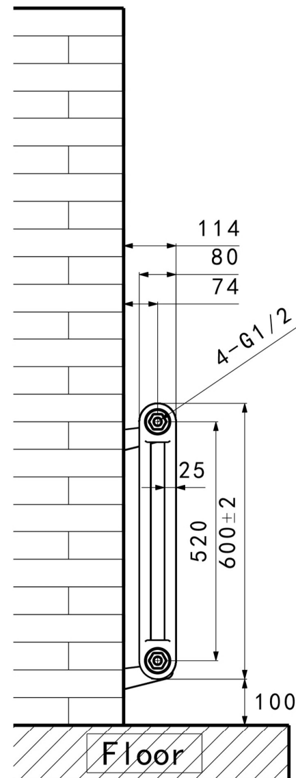
Side view
