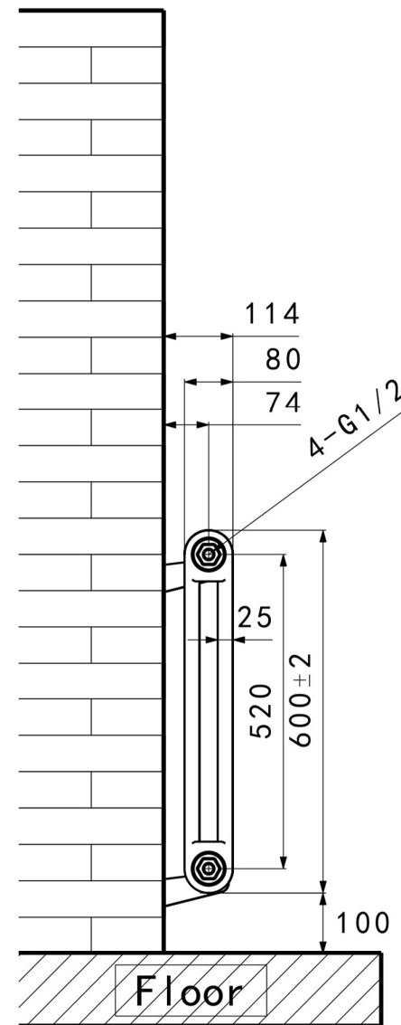
Side view
