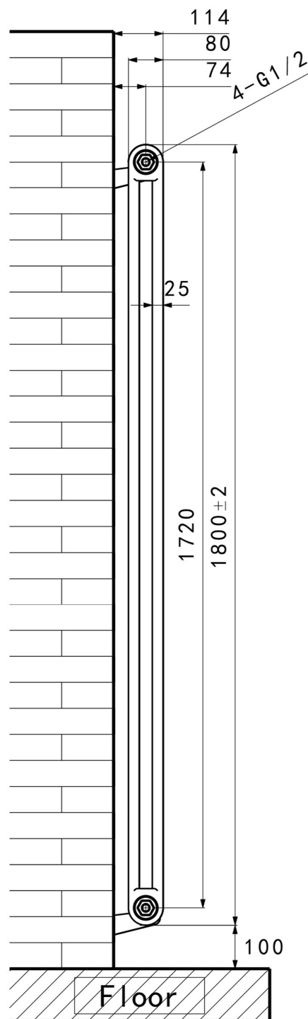
Side view
