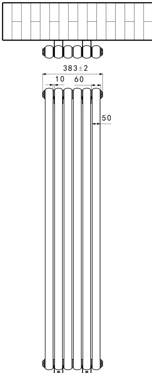
Top view
