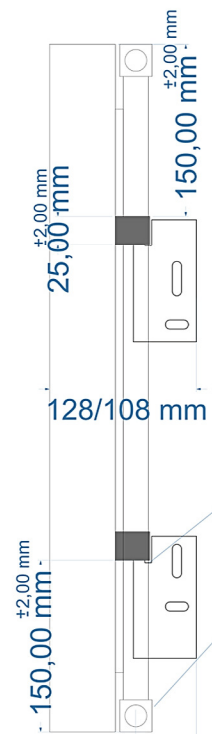
53,00/33,00 mm A SECTION ±2,00 mm
