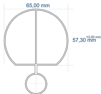
B SECTION
