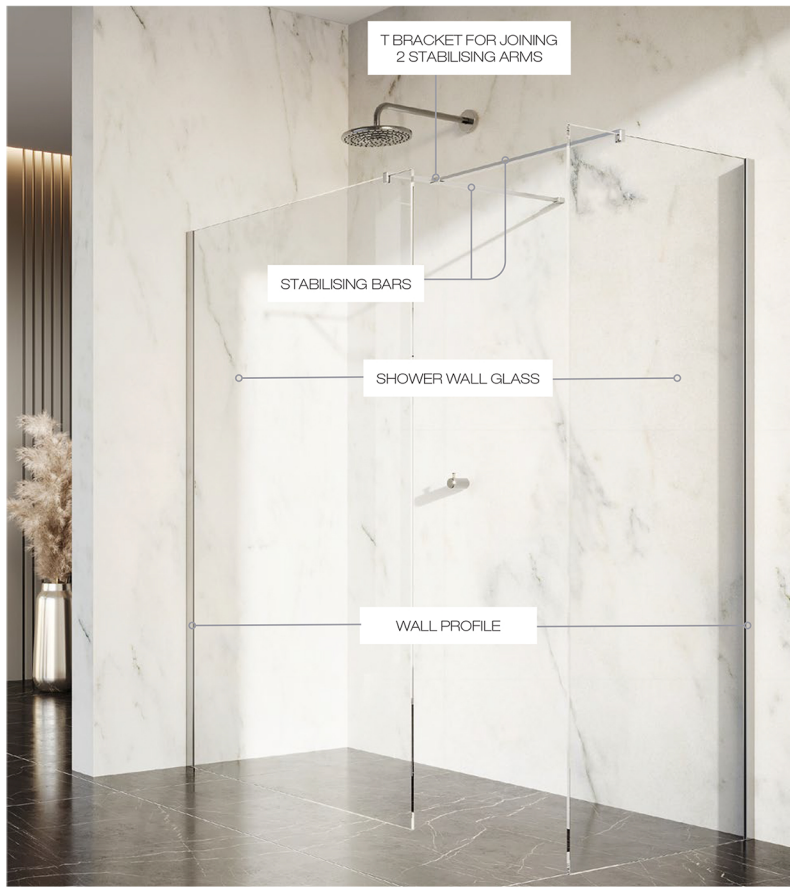
2 STABILISING BARS JOINED BY A T BRACKET
