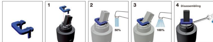
Volume Limiter
